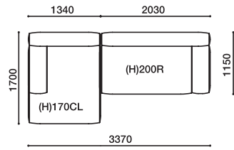
GLE-(H)170CL・(H)200R
