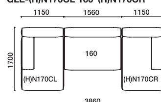
GLE-(H)N170CL·160·(H)N170CR
