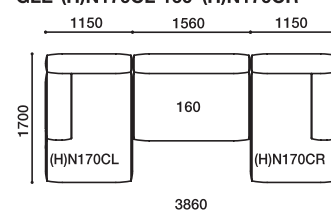
GLE-(H)N170CL・160・(H)N170CR
